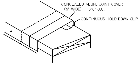
COPING ISOMETRIC
