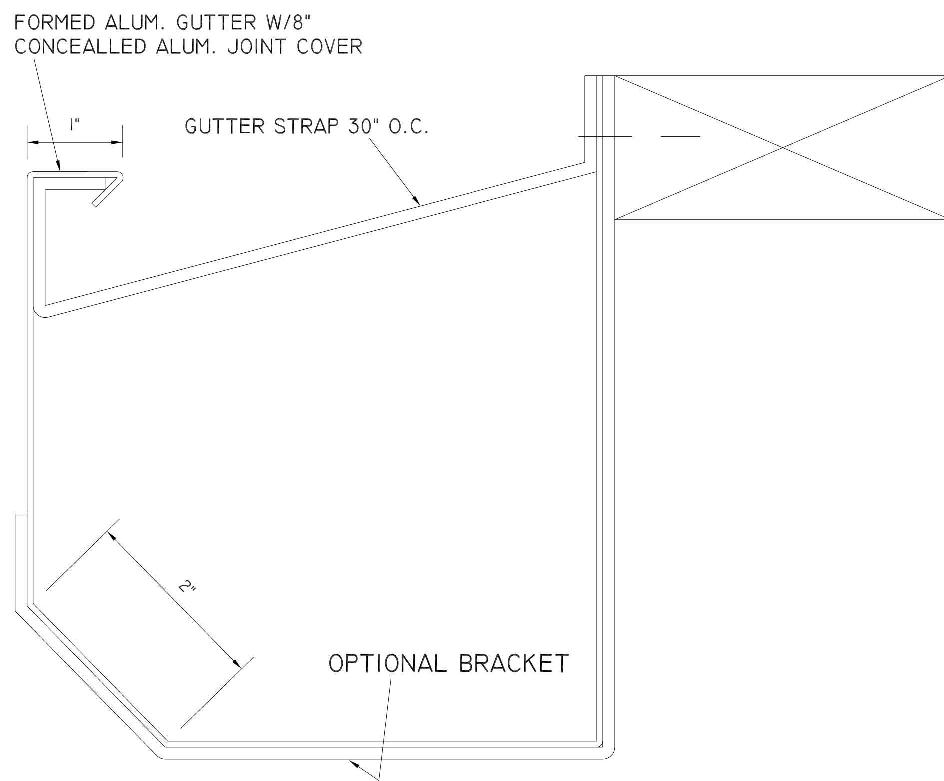
FORMED GUTTER
