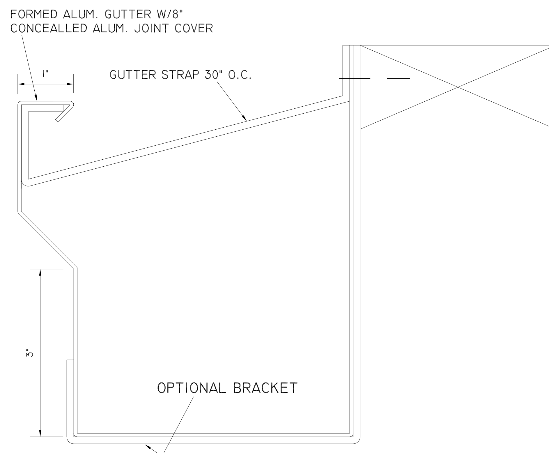
FORMED GUTTER
